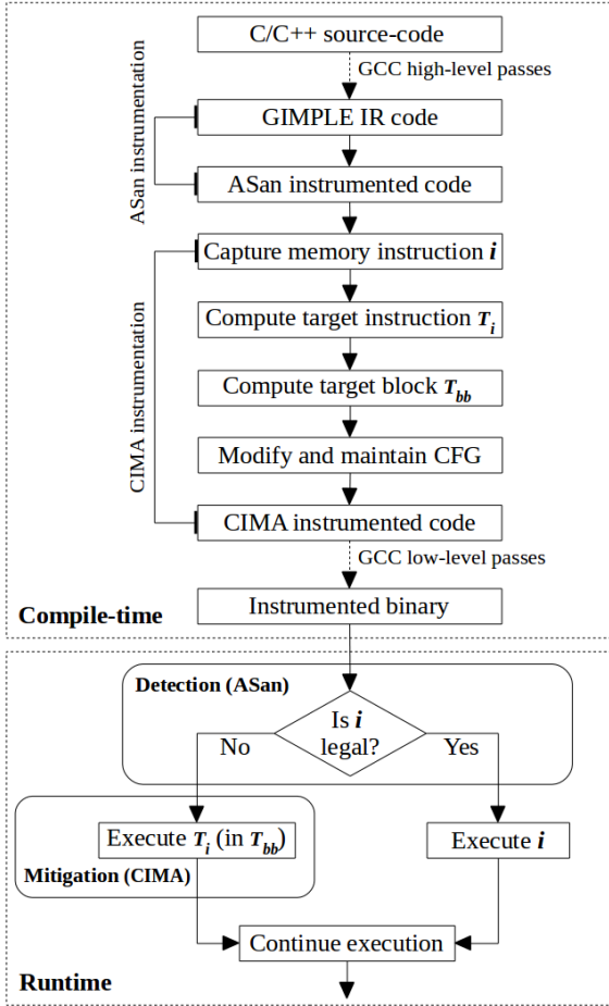
Figure 5: A high-level architecture of CIMA
