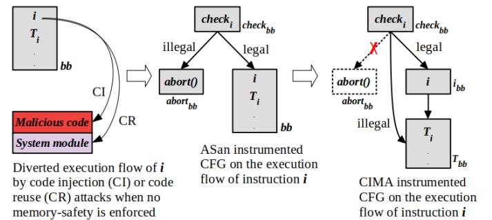
Figure 6: Illustrating the change of CFG in scenario 1 (i.e. i and T_i reside in same basic block) involving three cases: attacker diverted CFG (without memory-safety), ASan instrumented CFG (preventing exploitation but crashing execution) and CIMA instrumented CFG (preventing exploitation and continuing execution).
